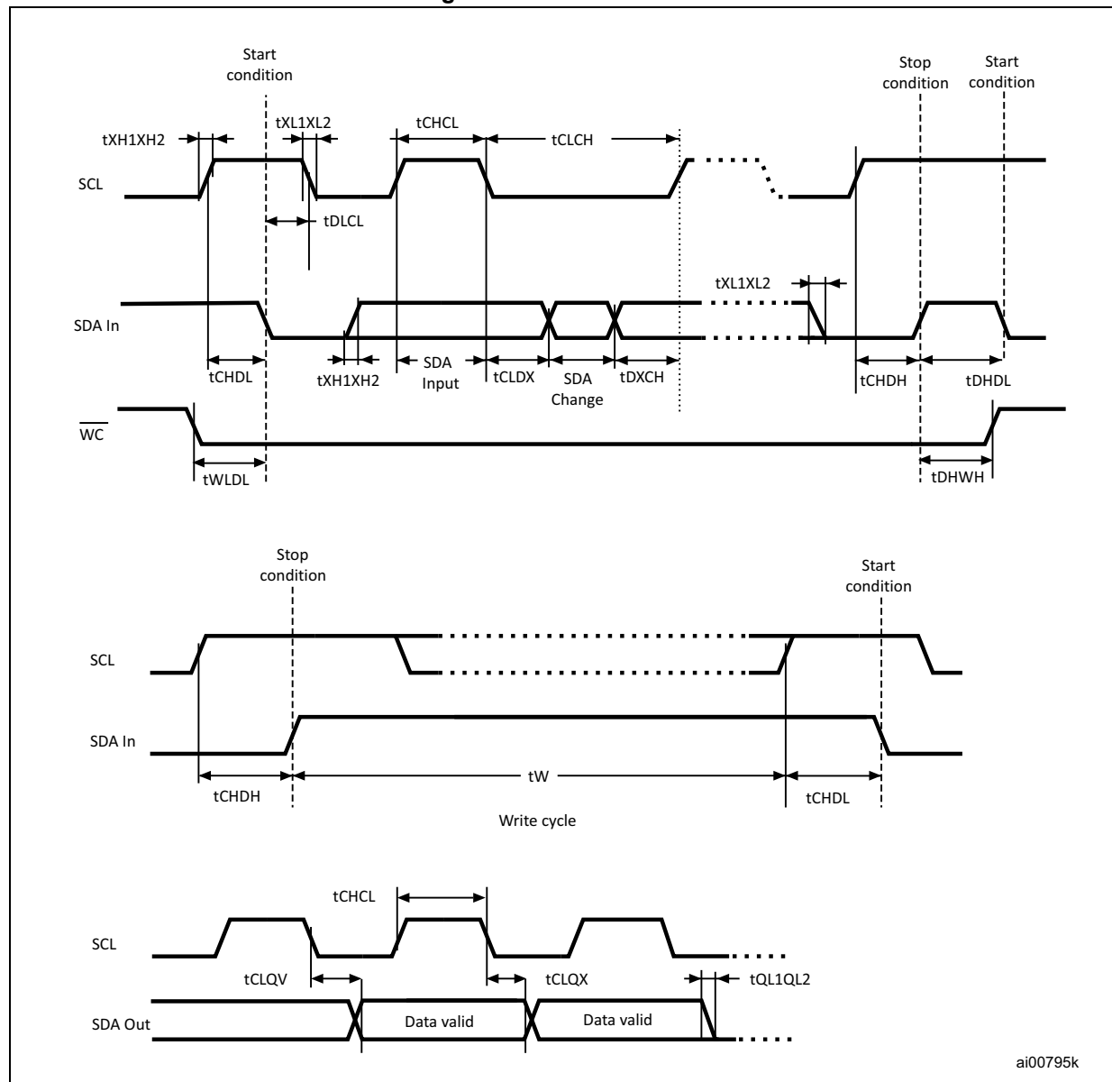
Figure 12. AC waveforms
