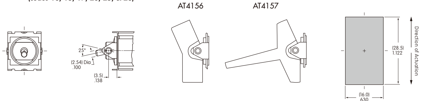
Large Actuators & Panel Cutouts for TZ Frame (actuator details on the following pages)
