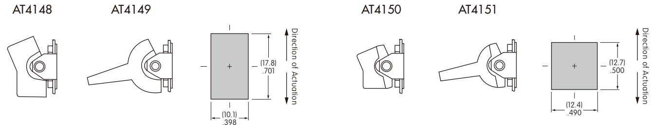
Small Actuators & Panel Cutouts for TX Frame (actuator details on the following pages)
