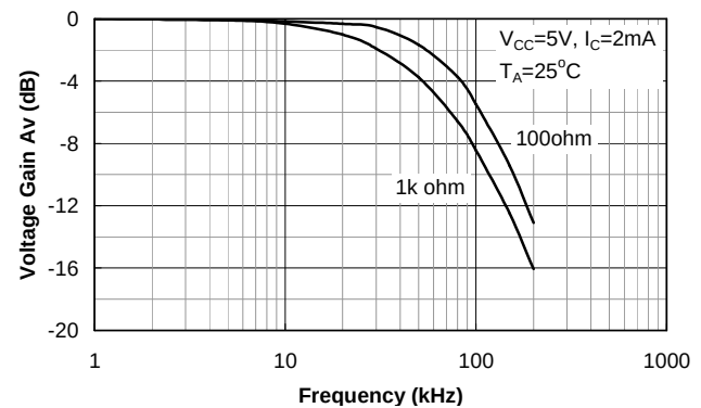
Figure 11. Frequency Response
