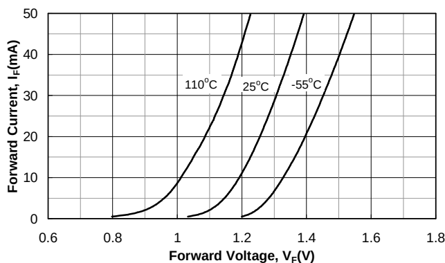
Figure 4. I_F vs. V_F
