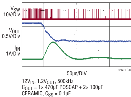
Single Phase Start-up with 25A
