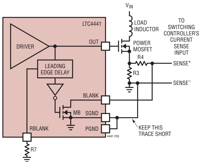
Figure 3. Blanking Circuit
