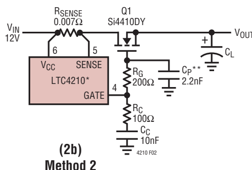
Figure 2. Frequency Compensation
