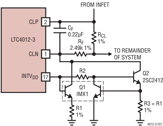
Figure 7. Adjusting Input Current Limit
