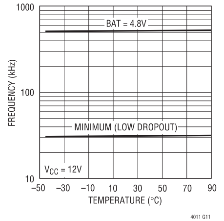
PWM Switching Frequency
