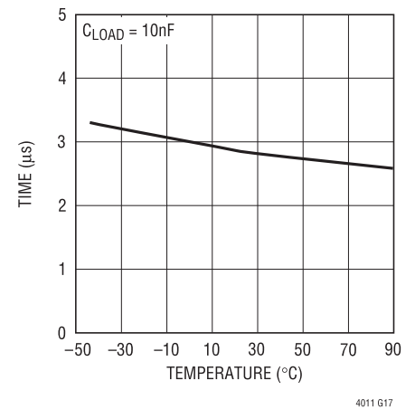
INFET OFF Delay Time
