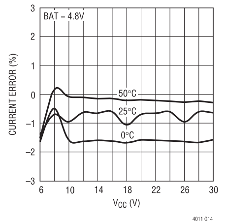
Fast Charge Current Line Regulation
