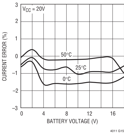
Fast Charge Current Output Regulation
