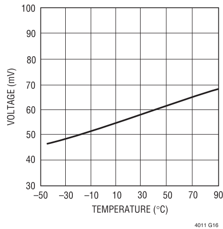
INFET Forward Regulation Voltage
