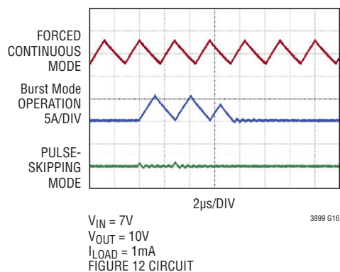
Inductor Current at Light Load (Boost)
