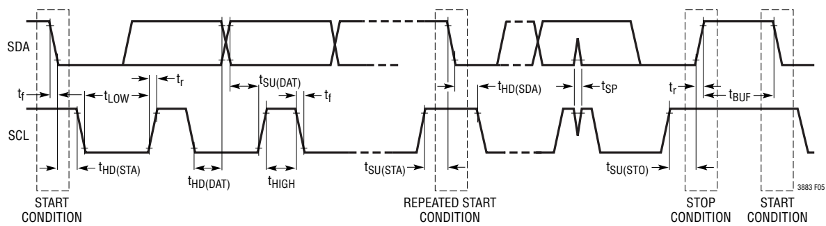
Figure 5. Timing Diagram
