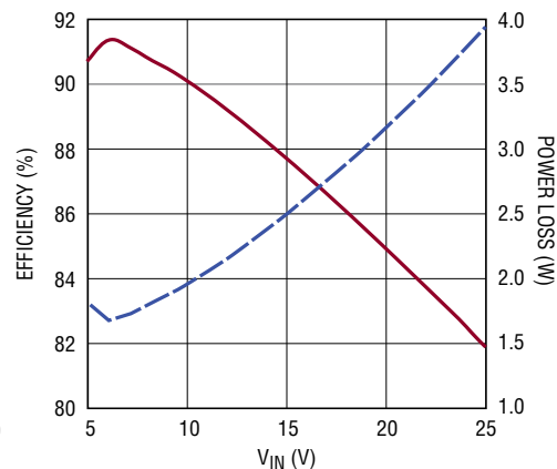
Efficiency and Power Loss vs Input Voltage (LTC3883)
