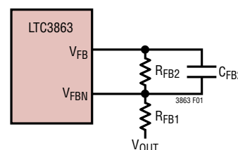
Figure 1. Setting the Output Voltage
