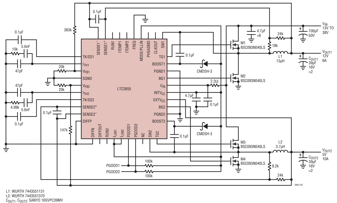
Figure 25. 12V, 6A and 5V, 10A Supply with DCR Sensing, f_{sw} = 250\text{kHz}
