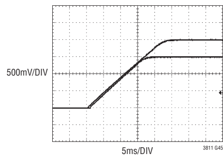
Coincident Tracking Start-Up
