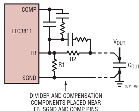
Figure 9. Output Divider and Compensation Component Placement
