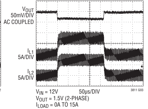
Load Step (Forced Continuous with Voltage Positioning)
