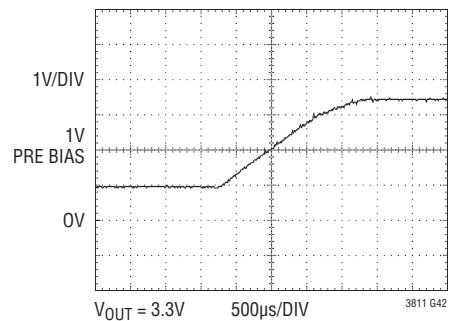
Start-Up Into a Pre-Biased Output Capacitor
