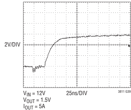
Bottom Gate Turn-On Waveform Driving Renesas RJK0301DPB
