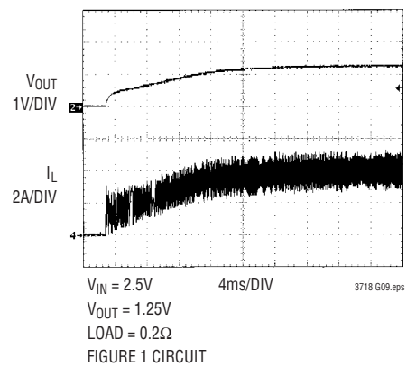
Start-Up Response
