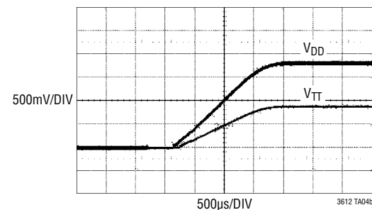
Ratiometric Start-Up
