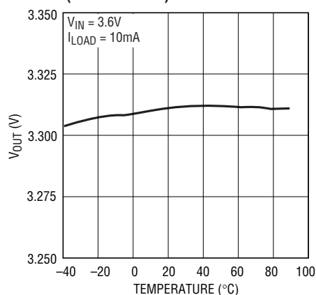
V_{\text{OUT}} Regulation vs Temperature (3.3V Version)
