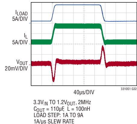
Load Transient Response Forced Continuous Mode
