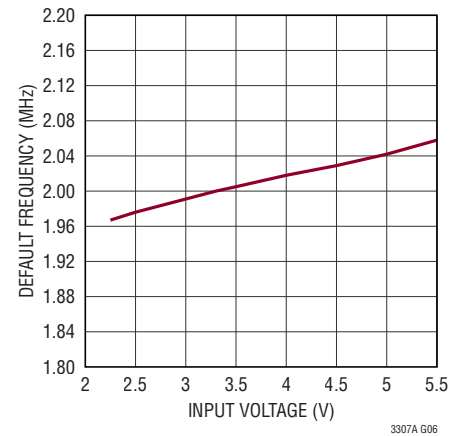
Default Switching Frequency
