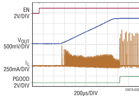
Start-Up Waveforms Burst Mode
