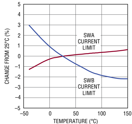
Inductor Current Limit Thresholds vs Temperature
