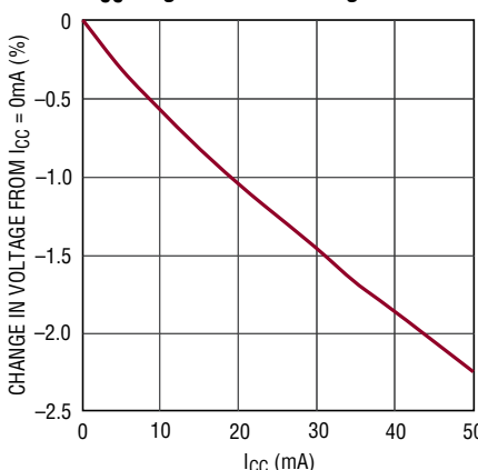
V_{CC} Regulator Load Regulation
