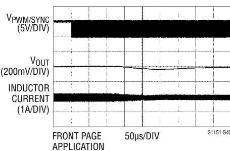
Phase-Locked Loop Acquisition, V_{IN} = 24\text{V} 1.2MHz Clock
