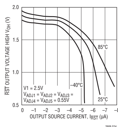
RST Output Voltage High vs RST Output Source Current LTC2908-C1
