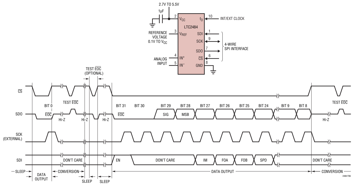
Figure 6. External Serial Clock, Reduced Data Output Length
