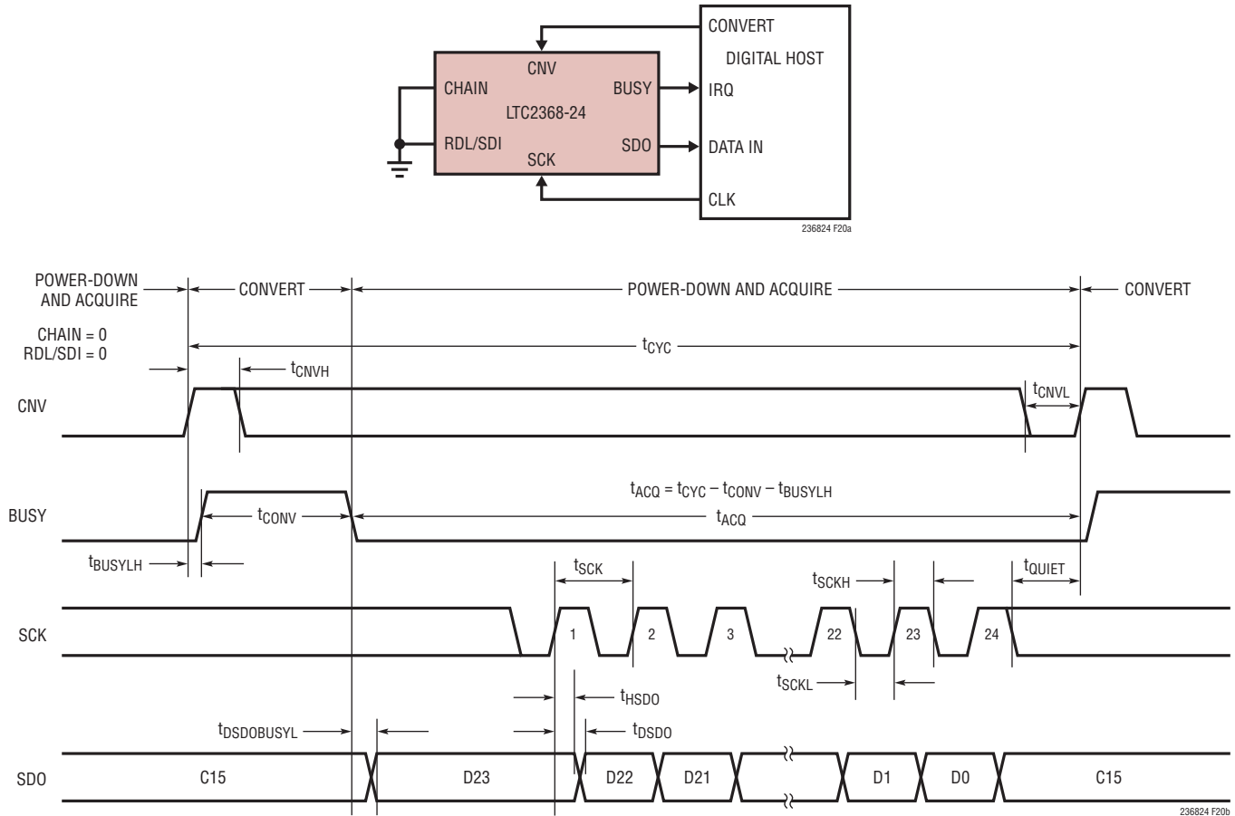
Figure 20. Using a Single LTC2368-24 in Normal Mode
