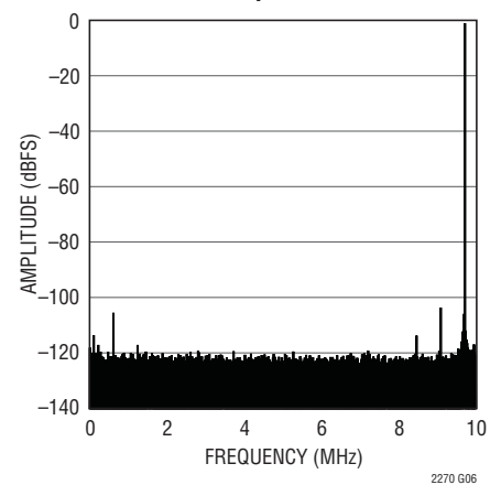
64k Point FFT, f_{IN} = 30.3\text{MHz} , -1dBFS, 20Msps
