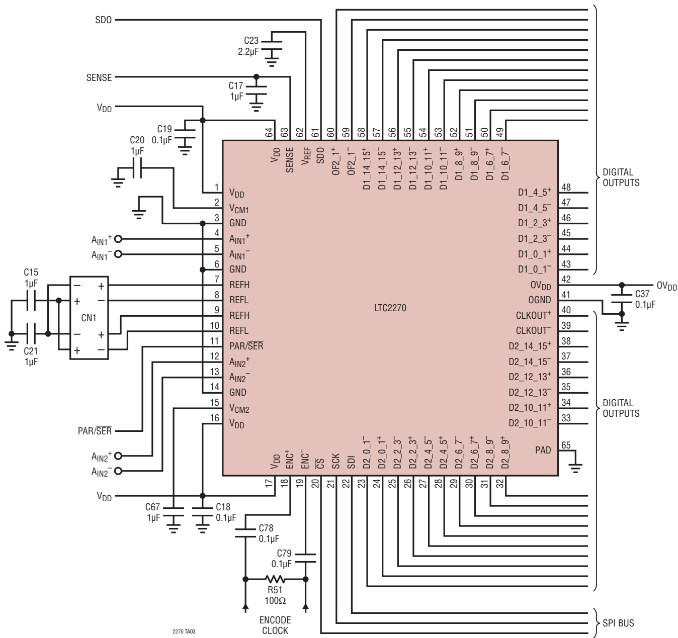
LTC2270 Schematic
