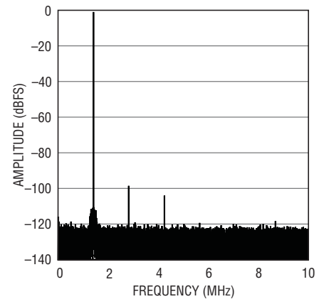
64k Point FFT, f_{IN} = 1.4\text{MHz} , -1dBFS, 20Msps
