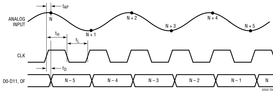
Timing Diagram
