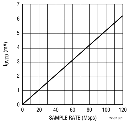
LTC2252: I_{OVD} vs Sample Rate, 5MHz Sine Wave Input, -1dB, OV_{DD} = 1.8\text{V}
