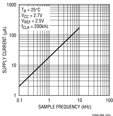
Supply Current vs Sample Rate
