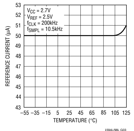
Reference Current vs Temperature
