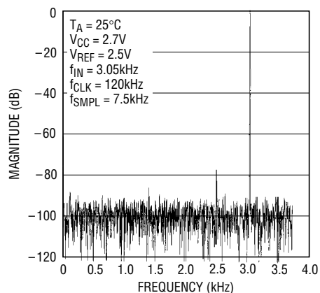
4096 Point FFT Plot
