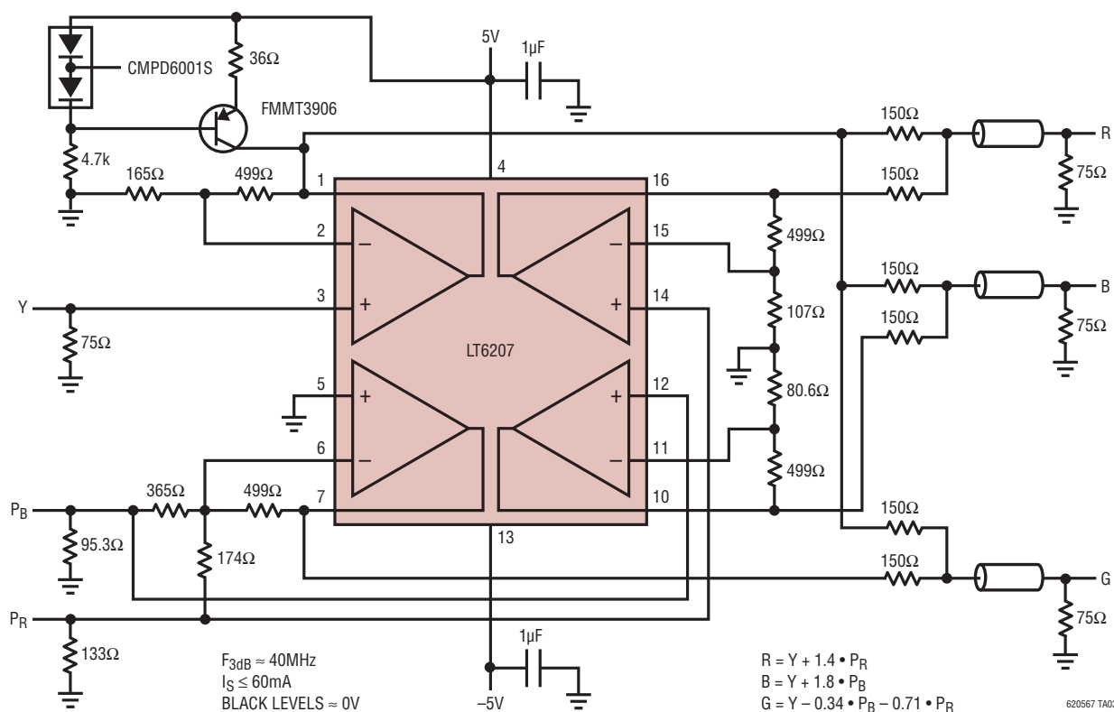
YPrP R to RGB Converter
