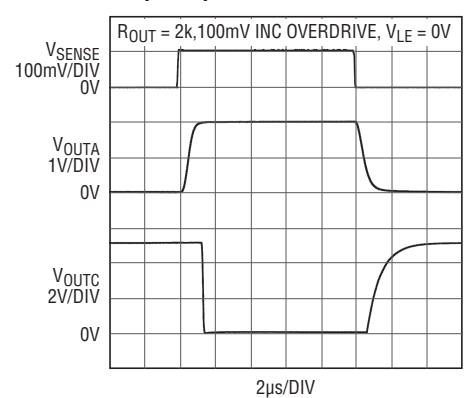
Step Response
