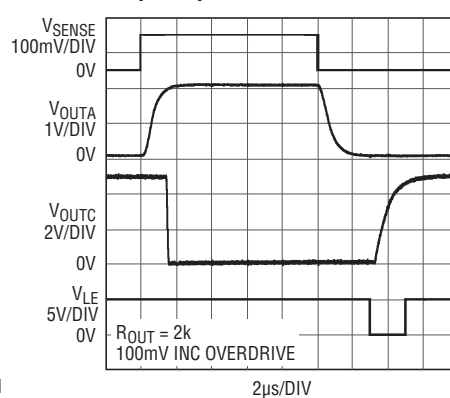
Step Response
