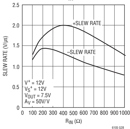
Slew Rate vs R_{IN}
