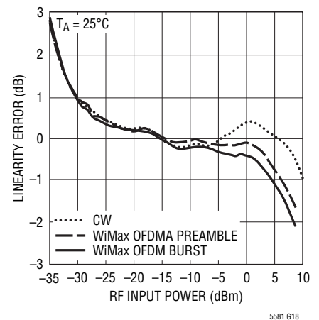
Linearity Error vs RF Input Power, 3.5GHz Modulated Waveforms
