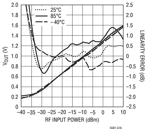
Output Voltage and Linearity Error at 3500MHz
