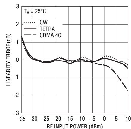
Linearity Error vs RF Input Power, 450MHz Modulated Waveforms
