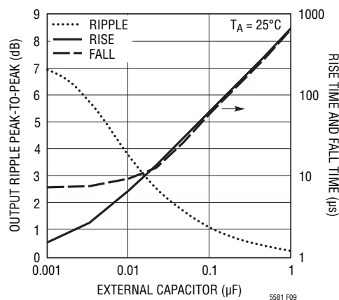
Figure 9. Residual Ripple, Output Transient Times for RF Pulse with WCDMA 4-Carrier Modulation vs External Filter Capacitor C4
