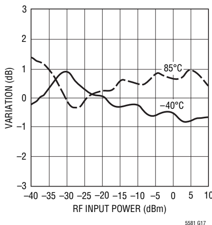
Linearity Error Temperature Variation from 25°C at 3500MHz
