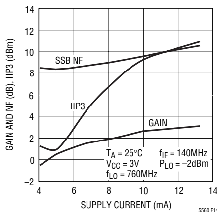
Figure 14. 900MHz Upconverting Mixer Gain, Noise Figure and IIP3 vs Supply Current
