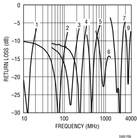
Figure 6. Input Return Loss vs Frequency for Different Matching Values
