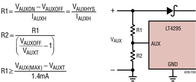
Figure 9. AUX Threshold and Hysteresis Calculation
