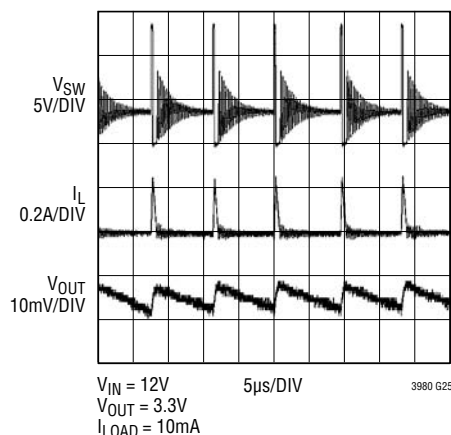
Switching Waveforms: Burst Mode Operation
