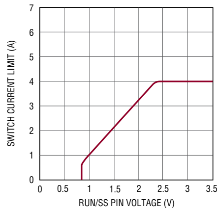
Soft-Start
