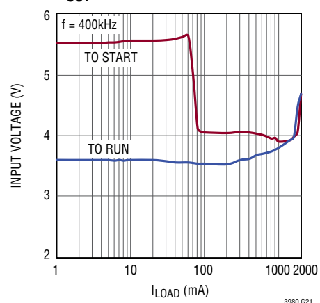
Minimum Input Voltage, V_{OUT} = 3.3\text{V}
