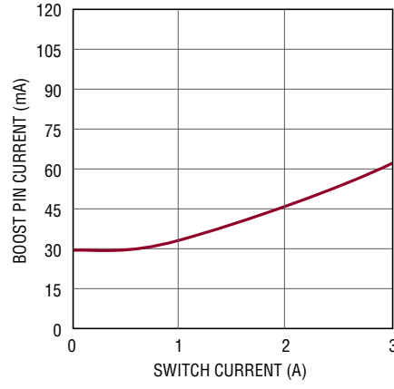
Boost Pin Current vs Switch Current
