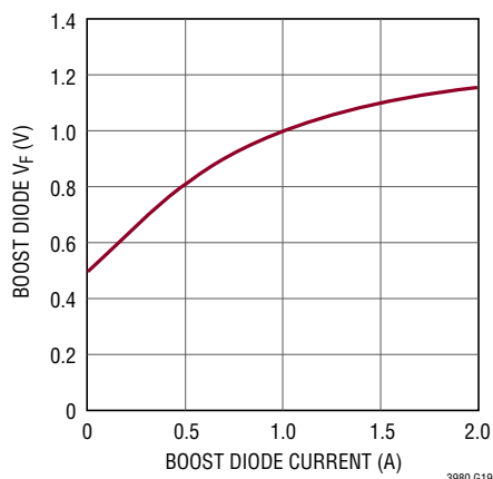
Boost Diode
