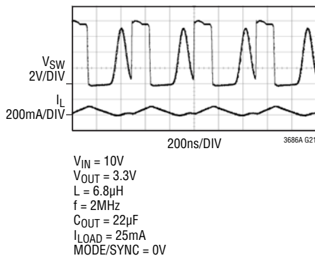
Light Load Discontinuous Mode Waveform
