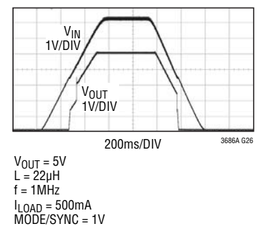
Start-Up Shutdown Waveform I_{LOAD} = 500\text{mA}
