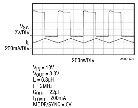
Continuous Mode Waveform
