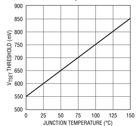
T_{SET} Pin Threshold vs Junction Temperature
