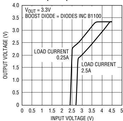
3.3V Dropout Operation
