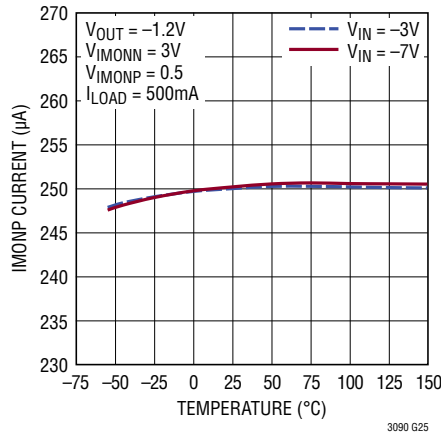
IMONP Pin Current at 500mA
