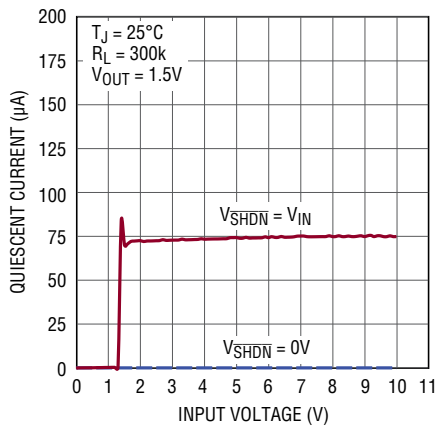
LT3065-1.5 Quiescent Current
