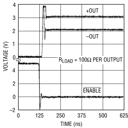
Turn-On Time
