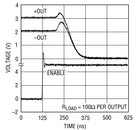
Turn-Off Time
