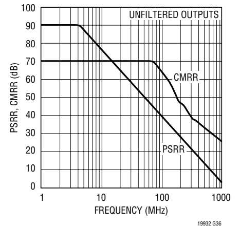
PSRR, CMRR vs Frequency
