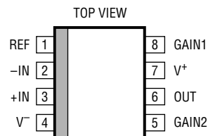
S8 PACKAGE 8-LEAD PLASTIC SO T_{JMAX} = 150^\circ\text{C} , \theta_{JA} = 190^\circ\text{C/W}
