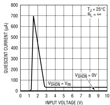
LT1962-3 Quiescent Current
