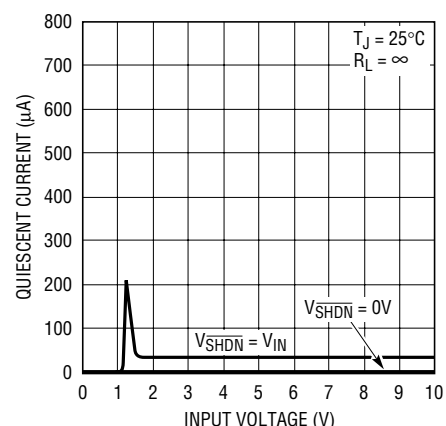
LT1962-1.5 Quiescent Current
