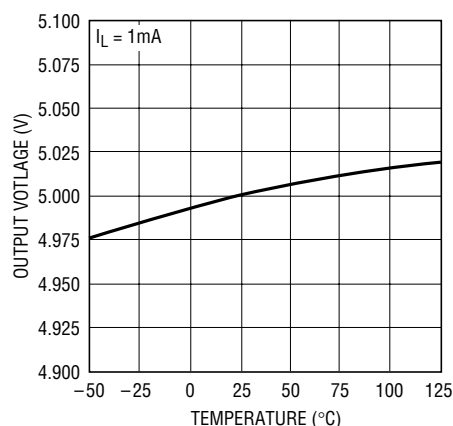
LT1962-5 Output Voltage
