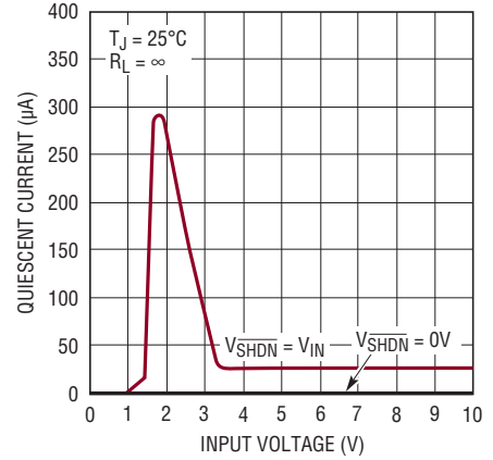
LT1762-3.3 Quiescent Current
