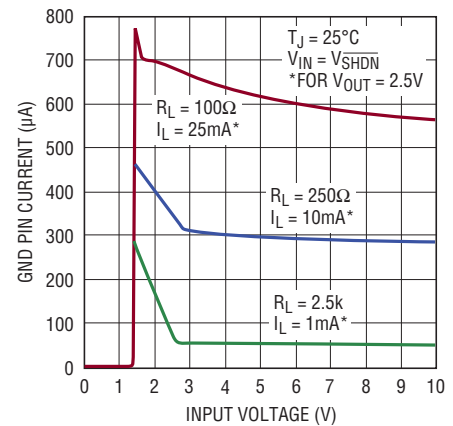
LT1762-2.5 GND Pin Current
