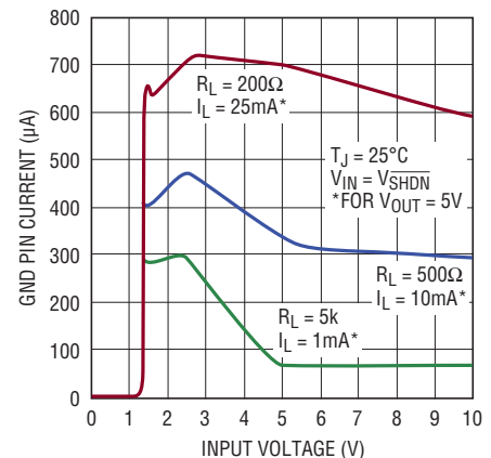
LT1762-5 GND Pin Current
