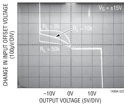
Open-Loop Gain
