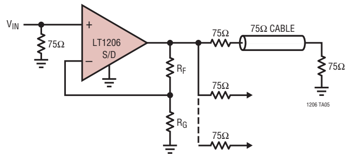
Distribution Amplifier
