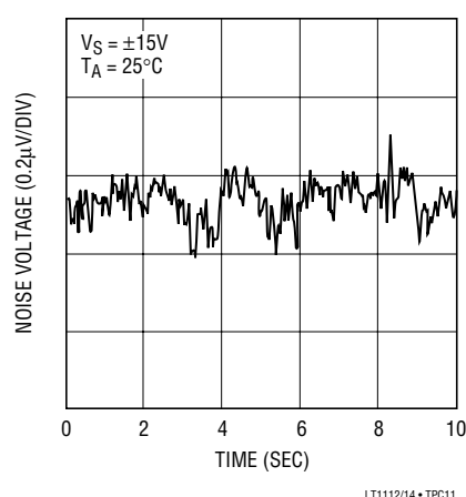
0.1Hz to 10Hz Noise
