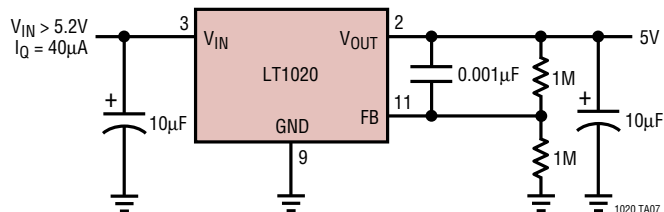
5V Regulator
