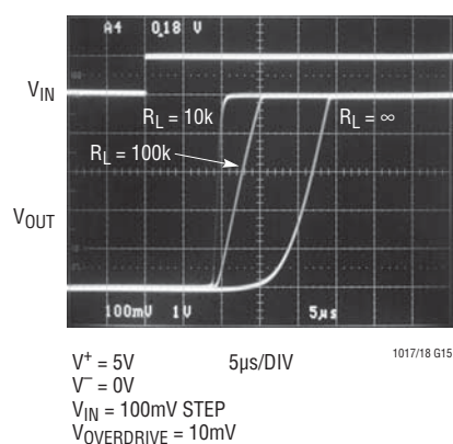
LT1017 Response Time
