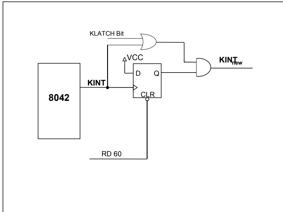
FIGURE 5 - KEYBOARD LATCH
