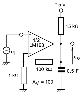
Figure 12: Low-frequency op amp (2)
