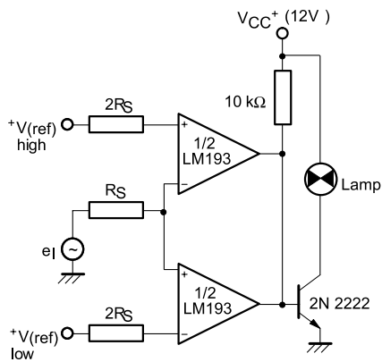
Figure 16: Limit comparator
