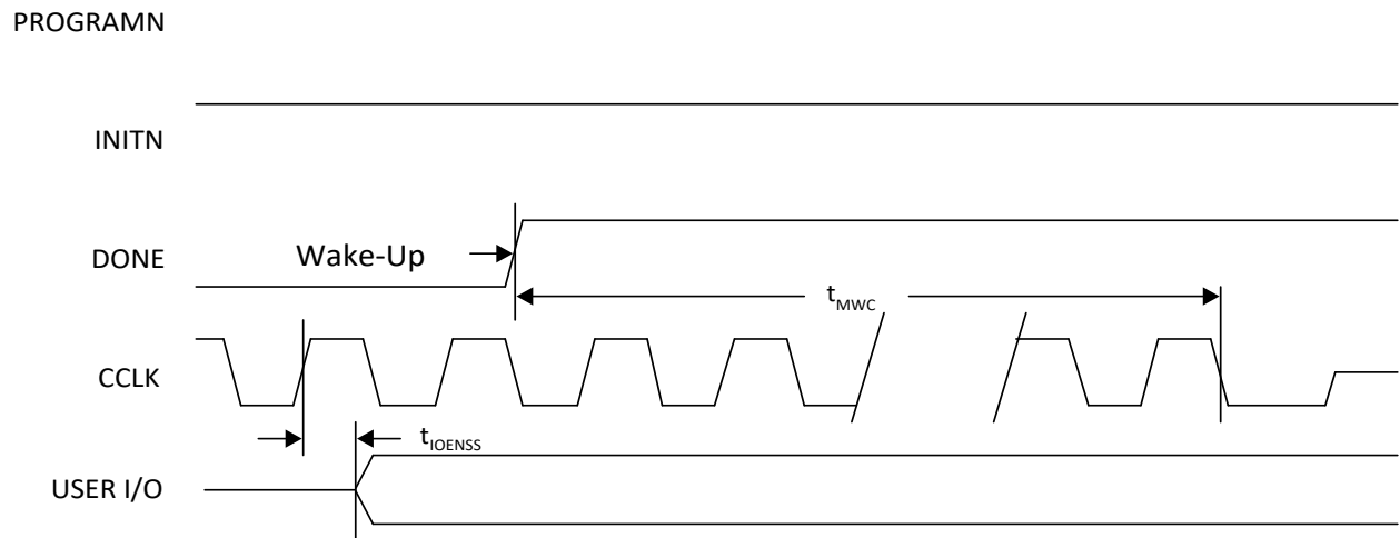
Figure 3.21. Wake-Up Timing
