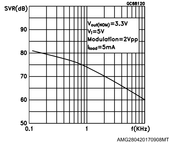
Figure 9: SVR vs frequency
